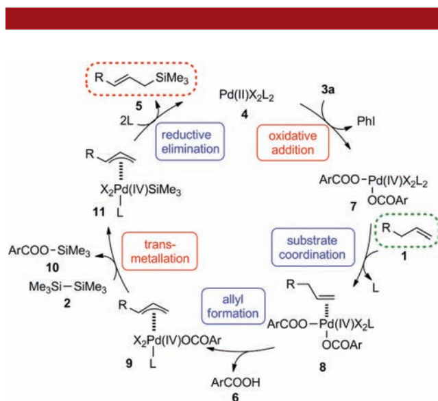
Figure 1. Plausible catalytic cycle (Ar = p -NO 2 -C 6 H 4 ).
